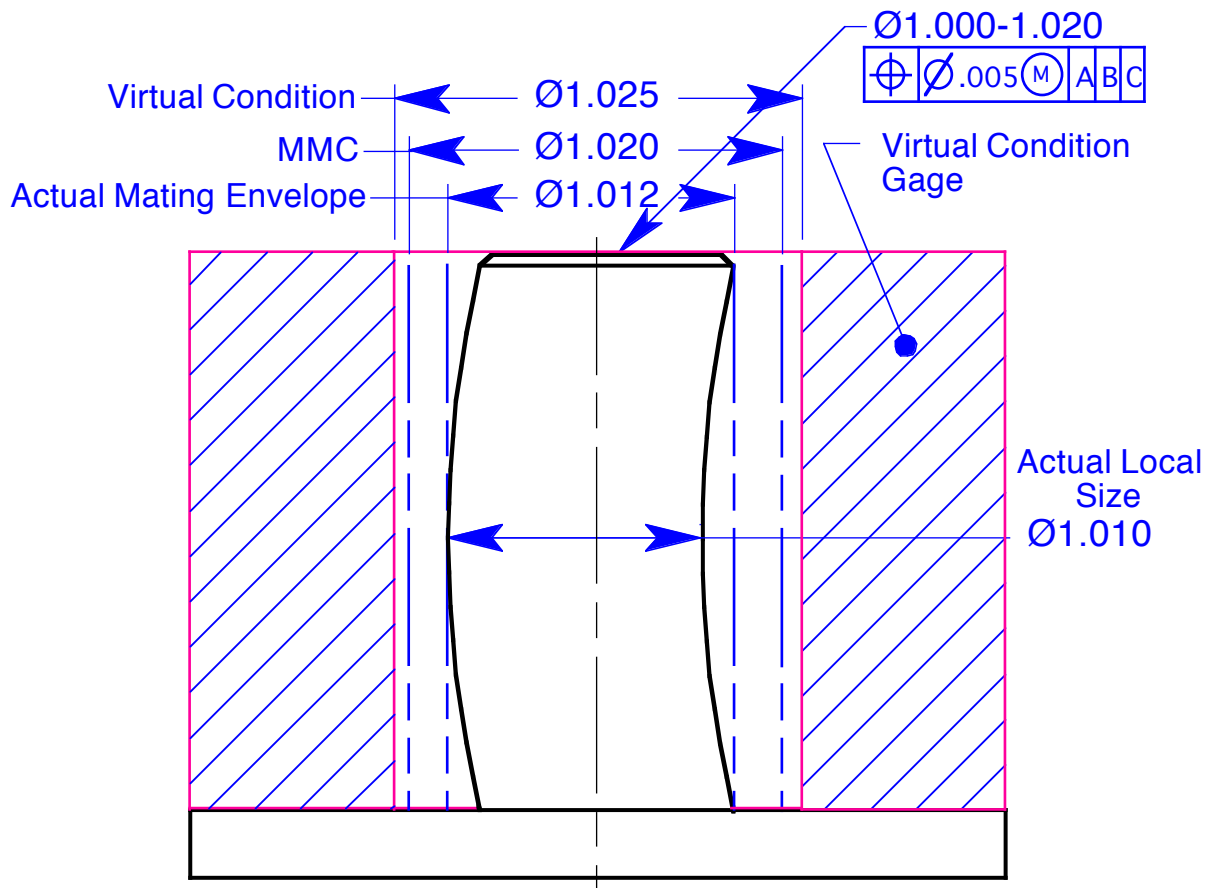
Figure 7-1 The actual local size, actual mating envelope, maximum material condition, and virtual condition
