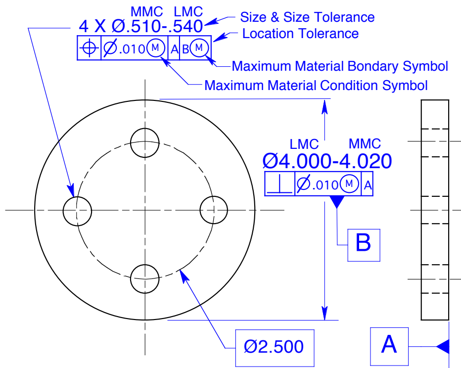
Figure 3-27 Maximum material condition and least material condition limits of size and material condition modifiers
