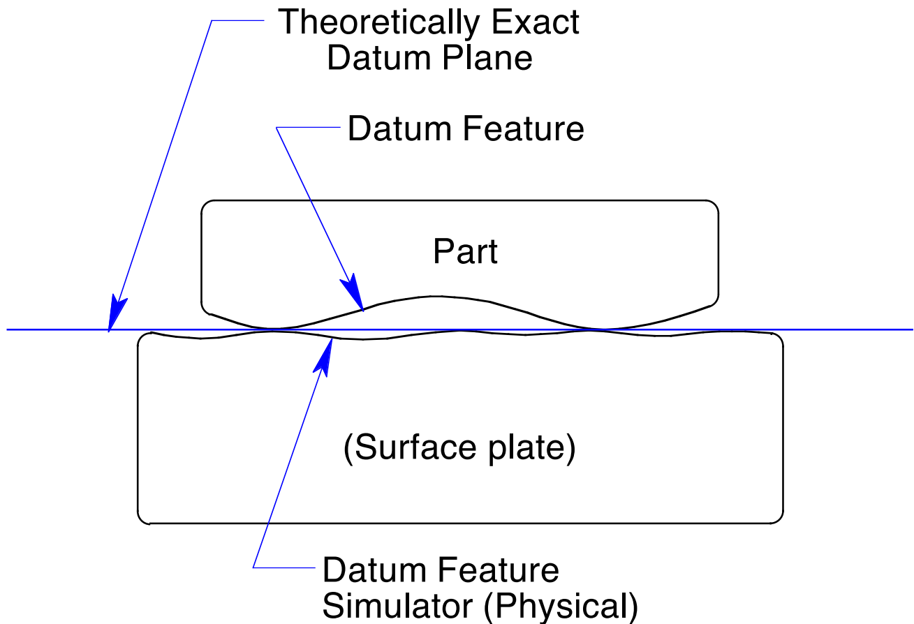
Figure 3-26 The relationship between a datum, a datum feature, and a physical datum feature simulator.
